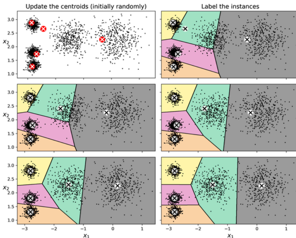
Figure 9-4. The k -means algorithm
