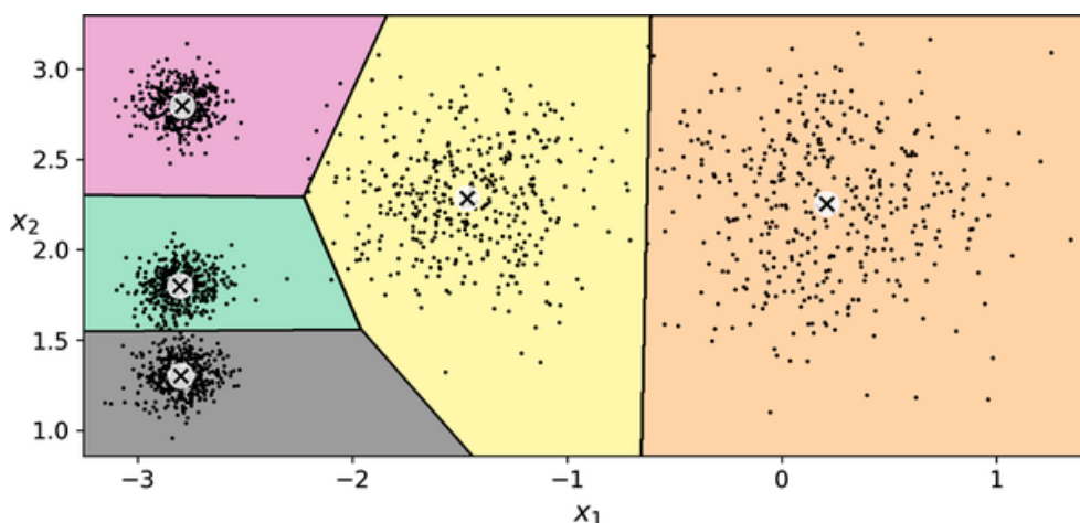
Figure 9-3. k-means decision boundaries (Voronoi tessellation)
