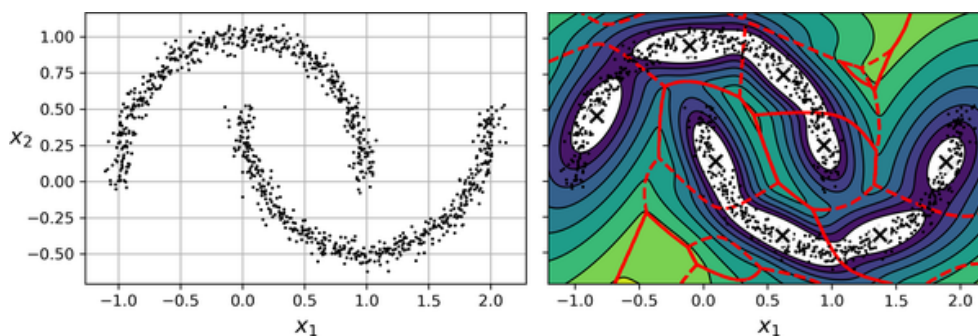
Figure 9-21. Fitting a Gaussian mixture to nonellipsoidal clusters
