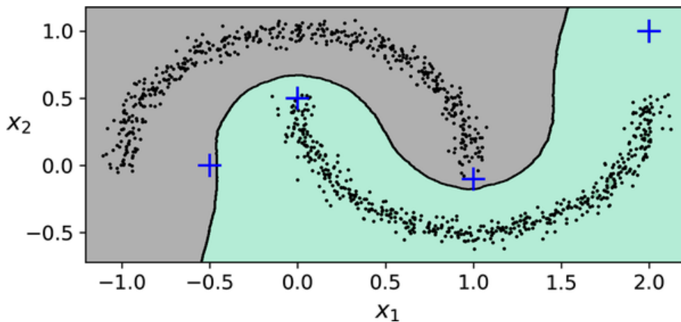
Figure 9-15. Decision boundary between two clusters
